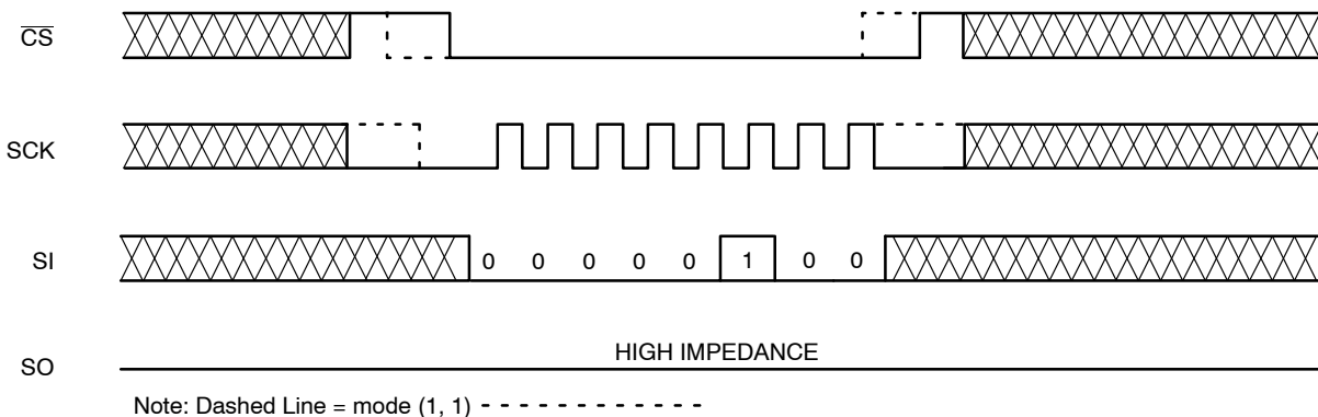
Figure 4. WRDI Timing
