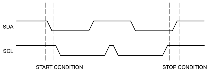
Figure 7. Start/Stop Condition
