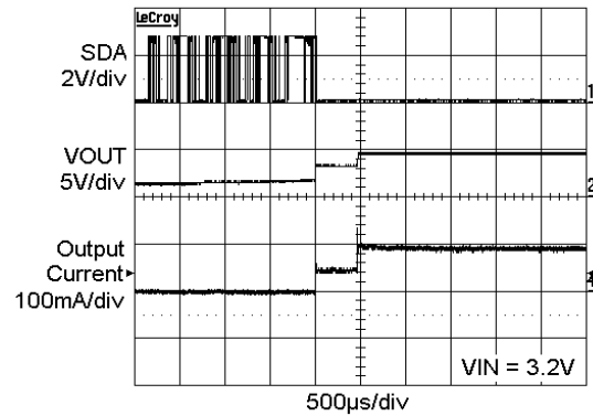
Figure 16. Power Up with 6 LEDs at 15\text{ mA} (1.5x Mode)
