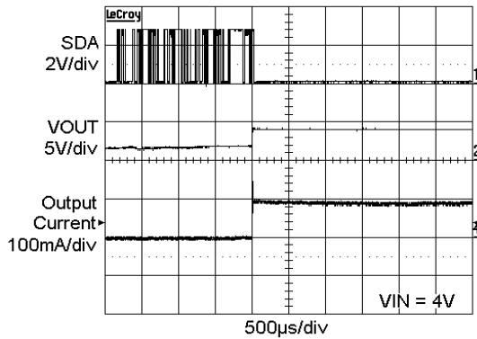
Figure 15. Power Up with 6 LEDs at 15\text{ mA} (1x Mode)
