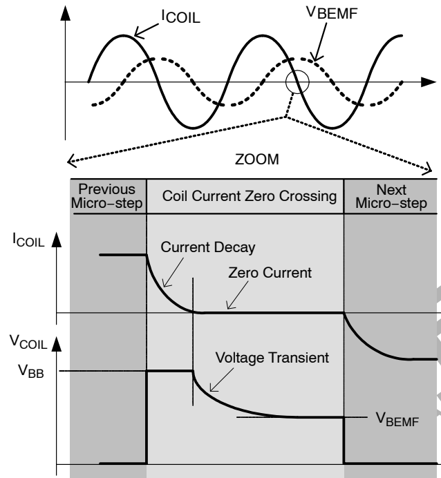
Figure 12. Principle of BEMF Measurement
