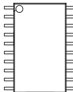
SOIC 20 IC SUFFIX CASE 751AQ
