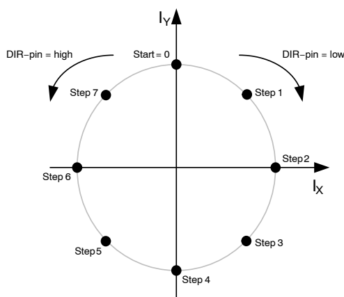
Figure 12. Half-step
