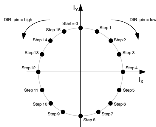
Figure 13. 1/4 Microstepping
