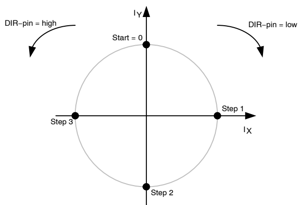
Figure 14. Full-Step 1/2 Rotated
