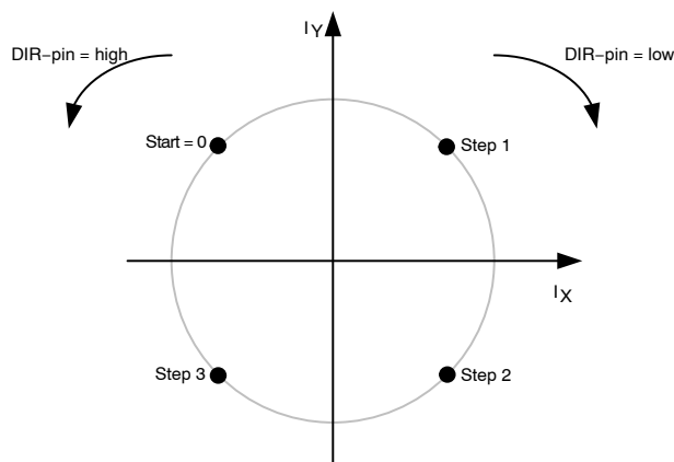
Figure 15. Full-step
