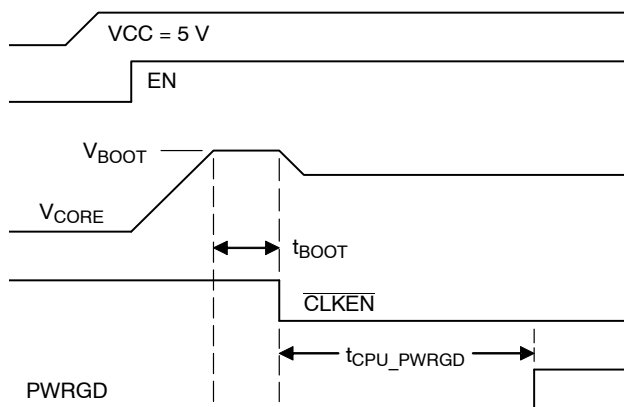
Figure 20. Powerup Sequence of APD3212/NCP3218/NCP3218G
