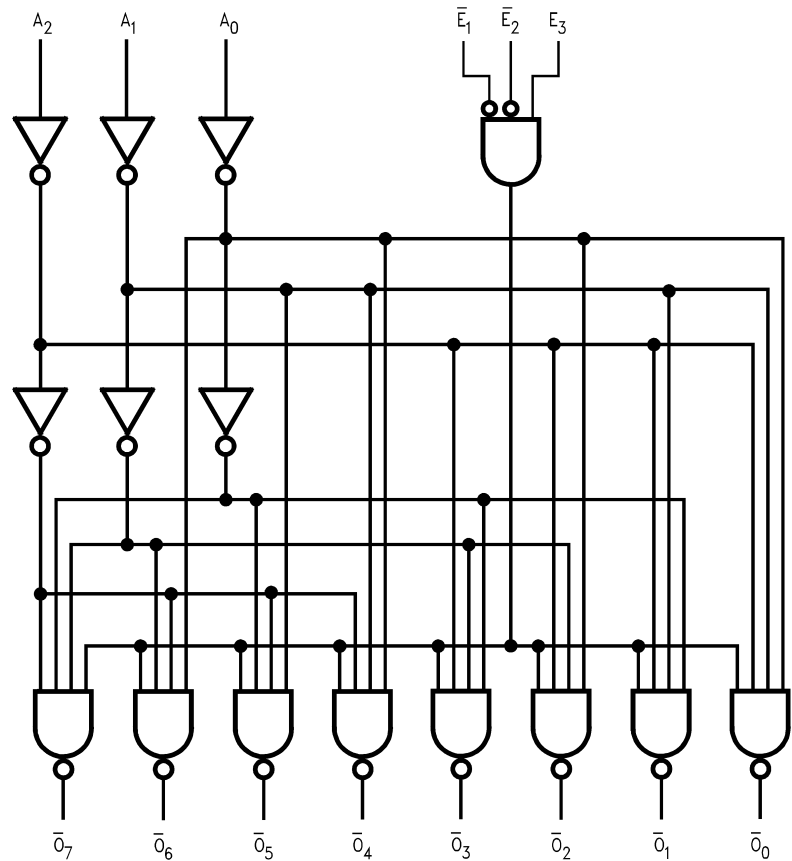
Figure 2. Logic Diagram
