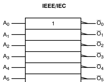
Figure 1. Logic Symbol
