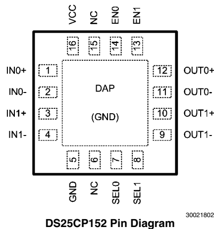
DS25CP152 Pin Diagram
