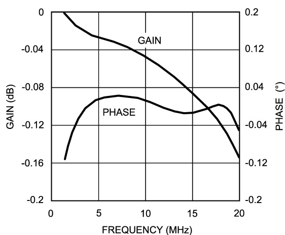
Gain Flatness &amp; Linear Phase
