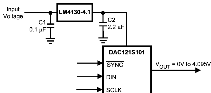
FIGURE 9. The LM4130 as a power supply
