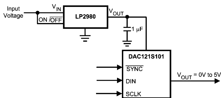
FIGURE 12. Using the LP2980 regulator
