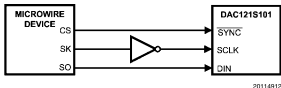
FIGURE 8. Microwire Interface
