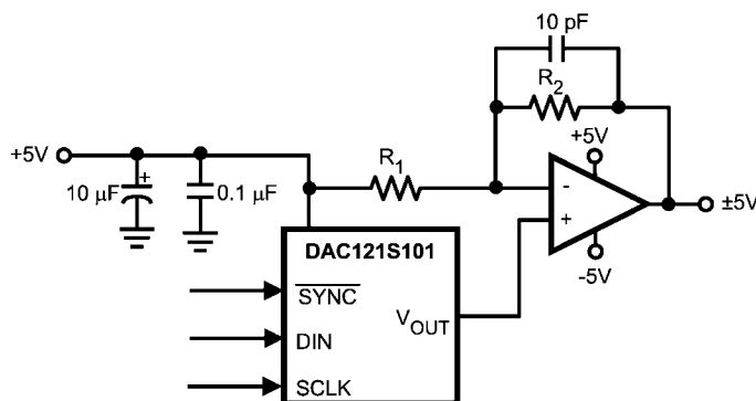
FIGURE 13. Bipolar Operation
