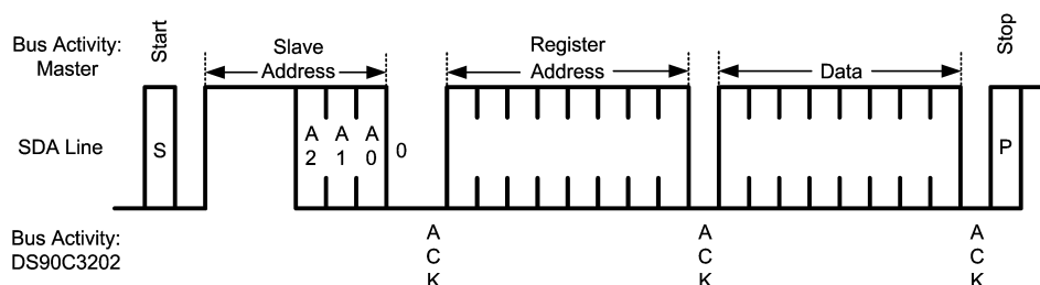
FIGURE 18. Byte Write
