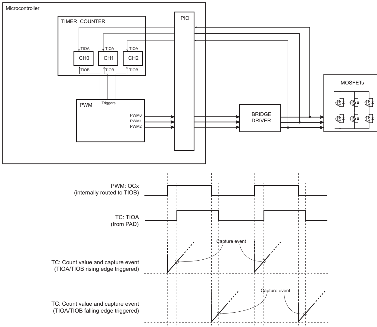
Figure 42-6. Triggering the TC: Delay Measurement
