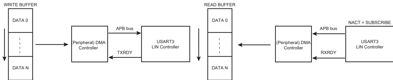
Figure 39-53. Slave Node with DMAC
