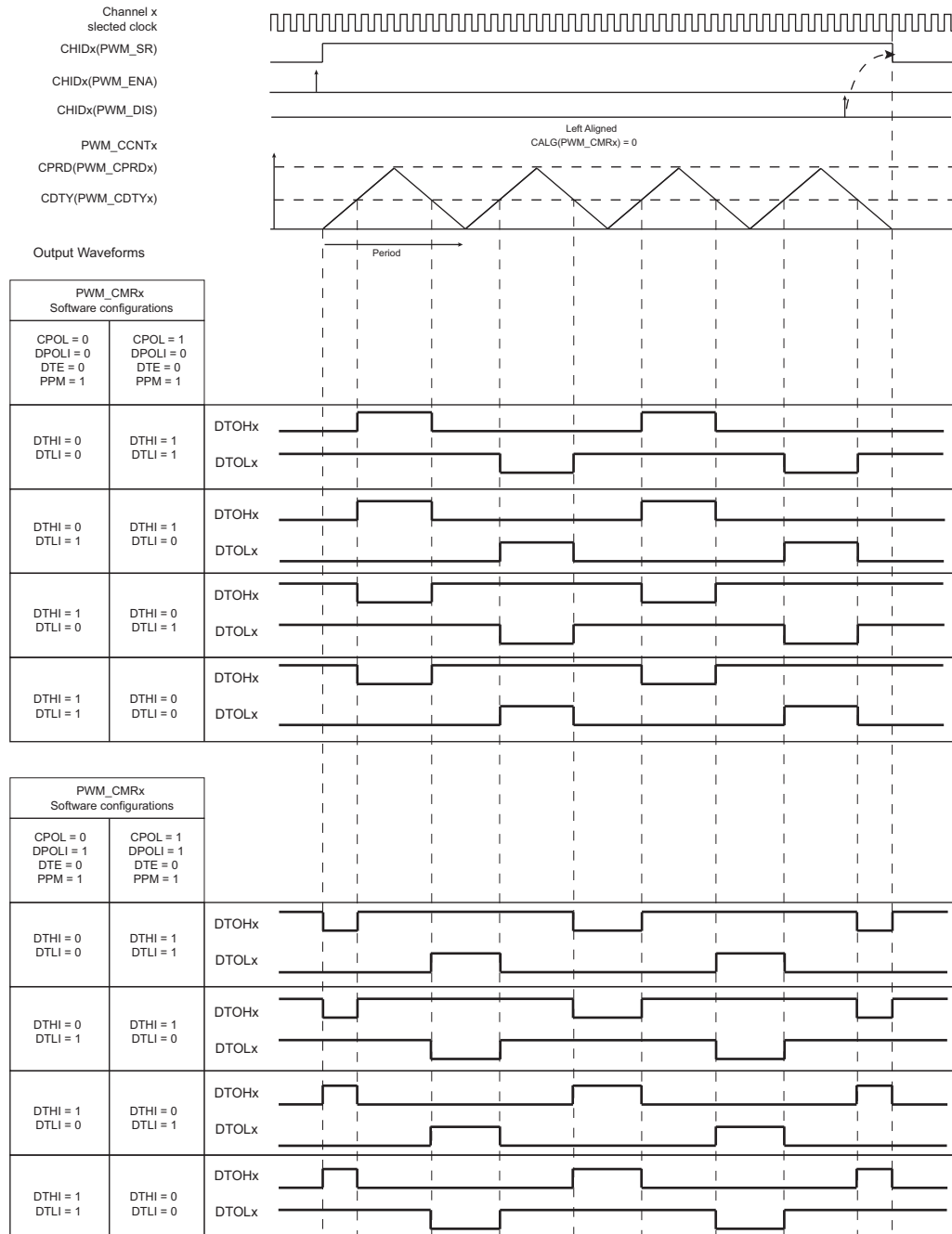
Figure 42-12. PWM Push-Pull Waveforms: Center-Aligned Mode
