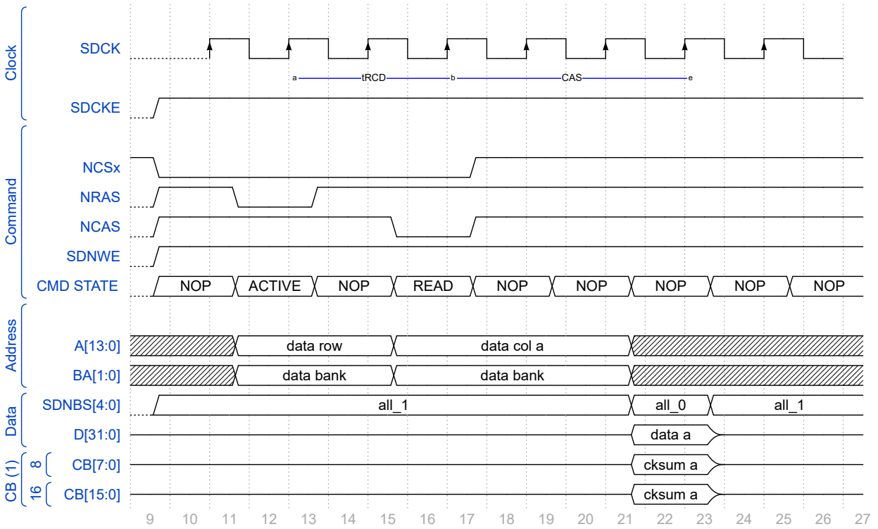
Figure 32-6. RD Burst 1 x 32 bits – 32 bits wide, HECC OFF/ON
