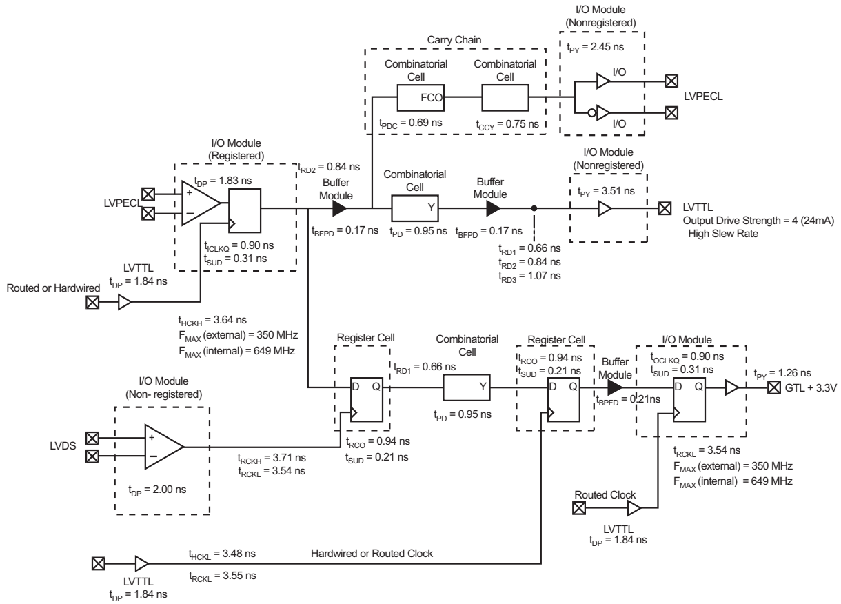
Figure 2-4 • Timing Model
