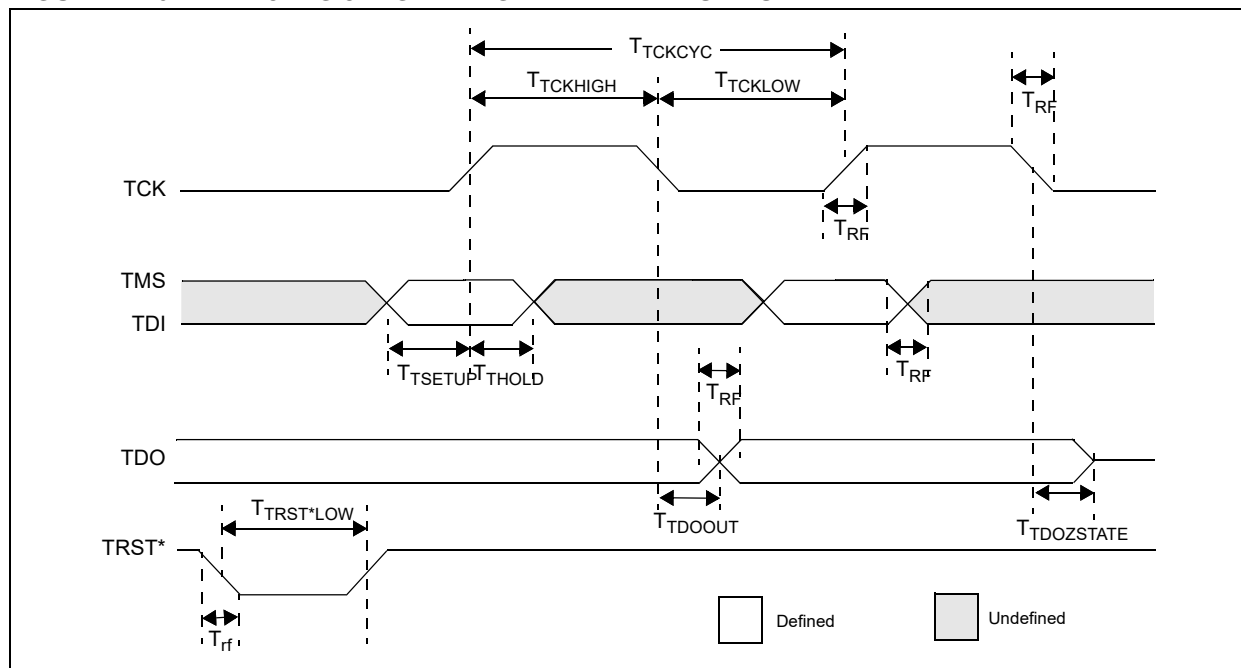
FIGURE 41-62: EJTAG/JTAG TIMING CHARACTERISTICS
