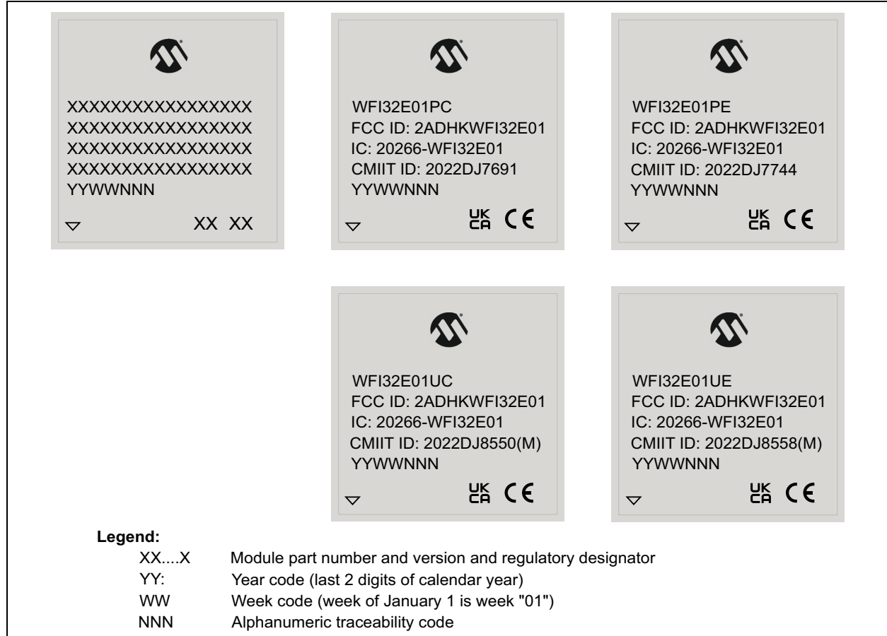
FIGURE 42-9: WFI32E01 MODULE PACKAGE MARKINGS
