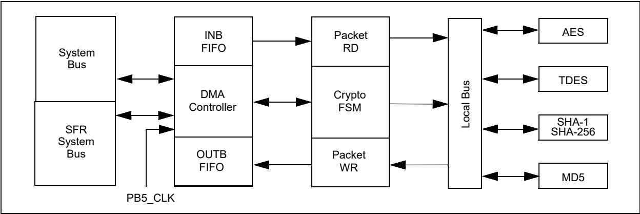
FIGURE 27-1: SYMMETRIC CRYPTO ENGINE BLOCK DIAGRAM
