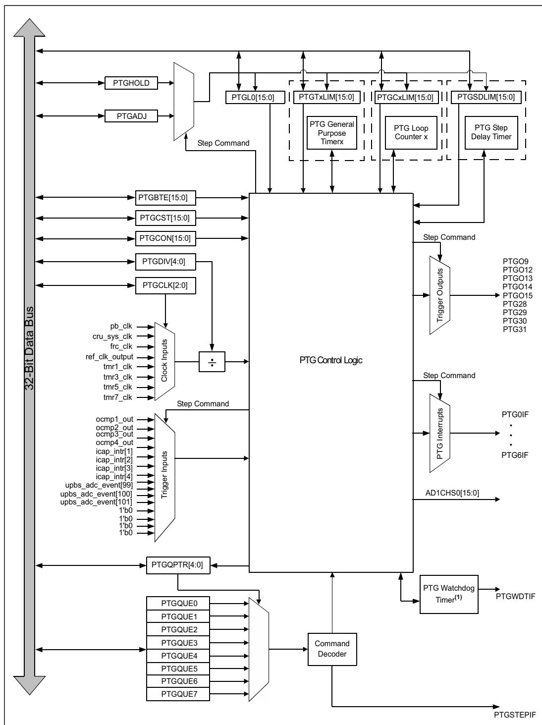
FIGURE 14-1: PTG BLOCK DIAGRAM
