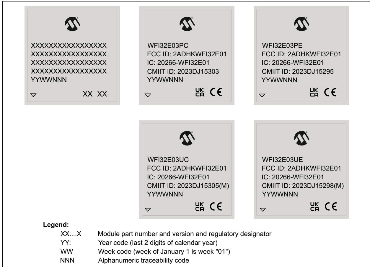
FIGURE 42-11: WFI32E03 MODULE PACKAGE MARKINGS
