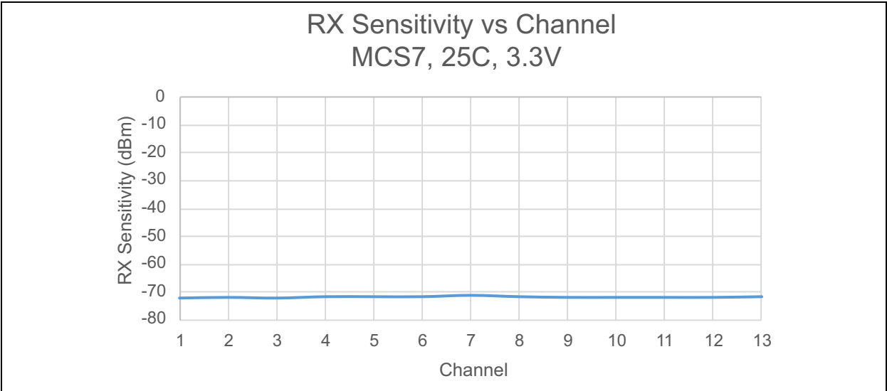
FIGURE 41-35: RX SENSITIVITY VS CHANNELS
