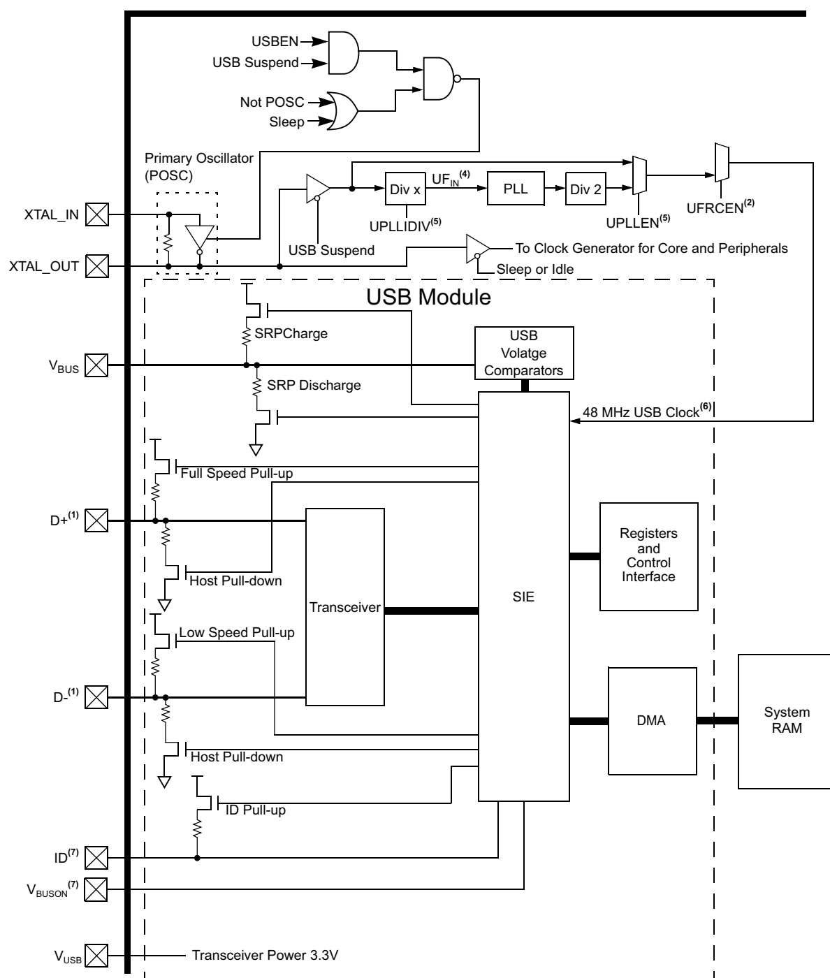
FIGURE 12-1: PIC32MZ W1 Family USB INTERFACE DIAGRAM
