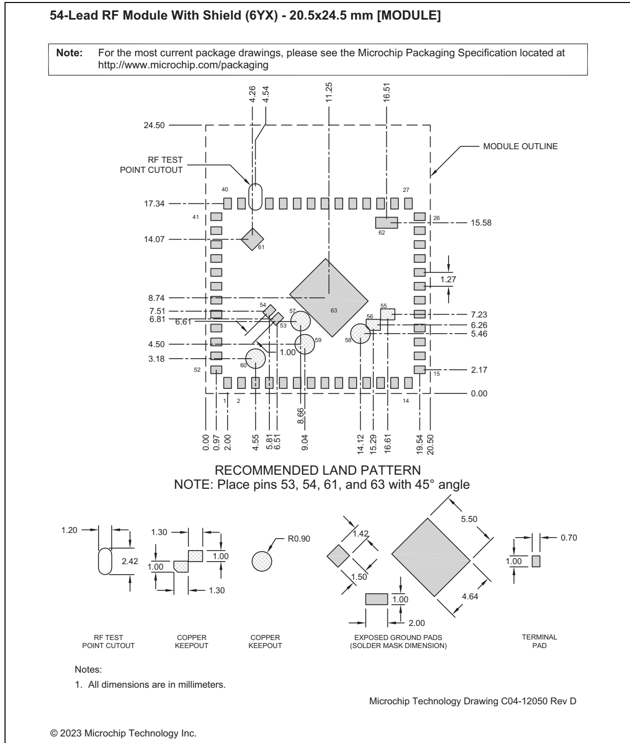
FIGURE 42-17: WFI32E01/WFI32E03 RECOMMENDED MODULE FOOTPRINT ON THE HOST BOARD
