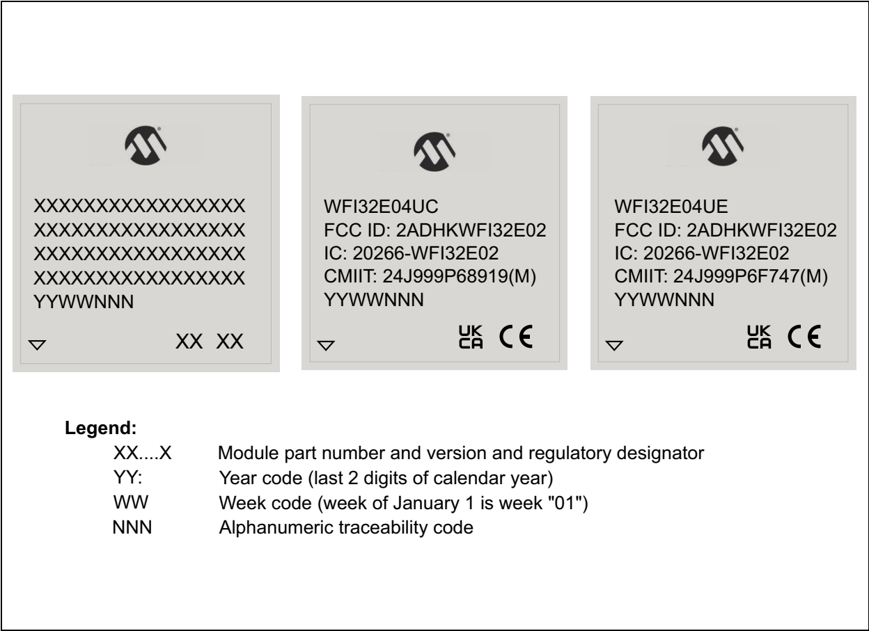
FIGURE 42-12: WFI32E04 MODULE PACKAGE MARKINGS
