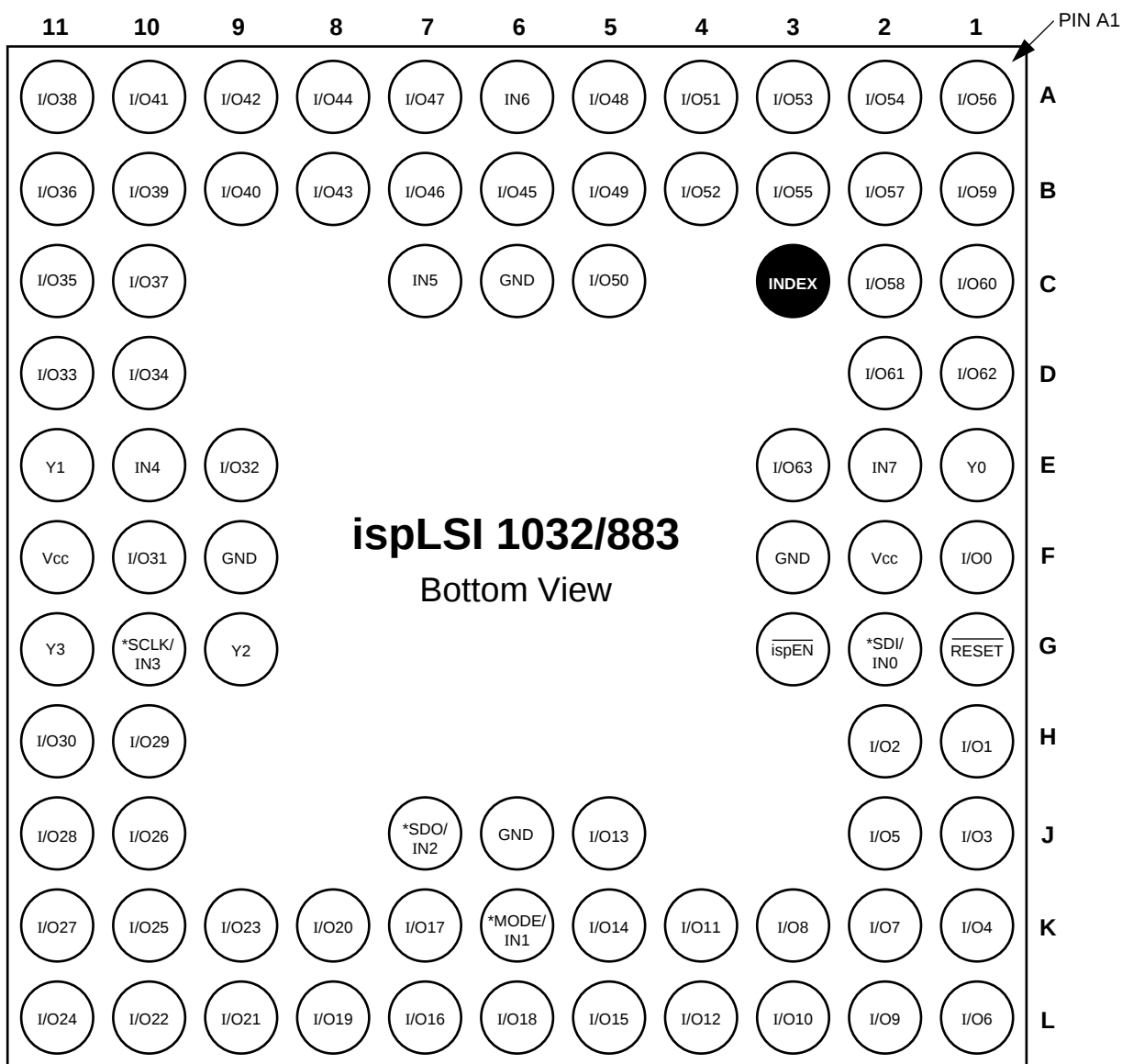
ispLSI 1032/883/883 84-Pin CPGA Pinout Diagram
