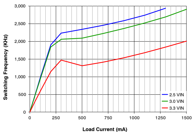
Figure 14. Frequency vs. Load Current and Input Voltage
