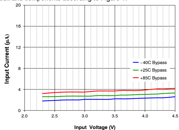
Figure 12. Quiescent Current vs. Input Voltage and Temperature, V_{OUT} = 3.15\text{ V} , Forced Bypass Mode
