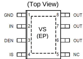
SO-8EP (Type E)
