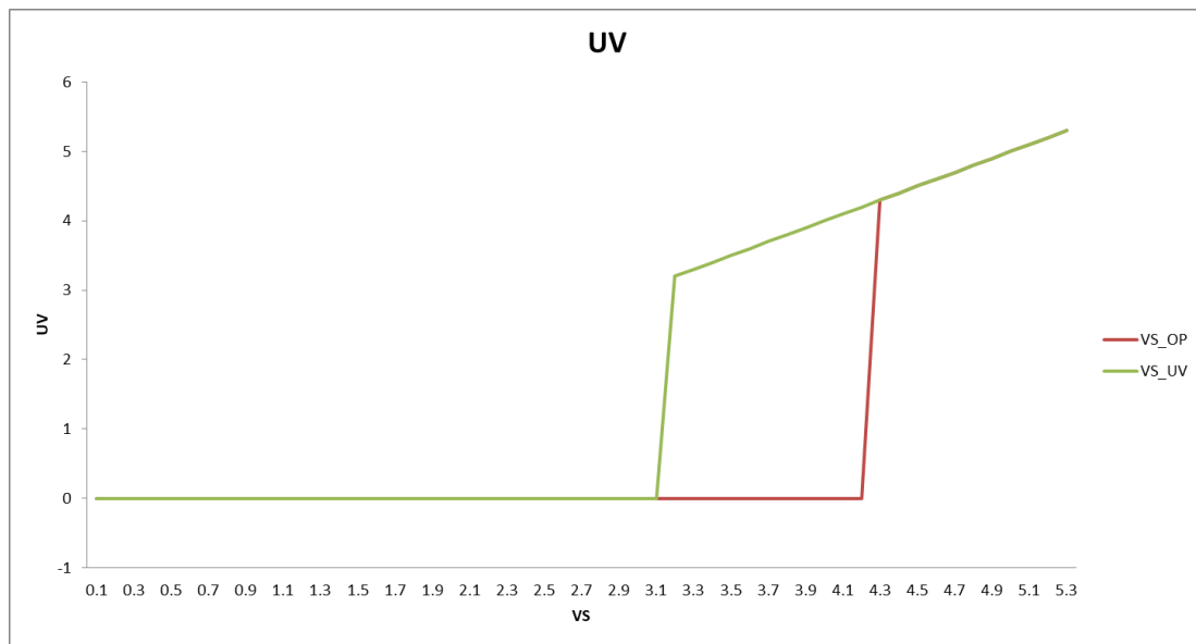
Figure 9. Undervoltage Behavior
