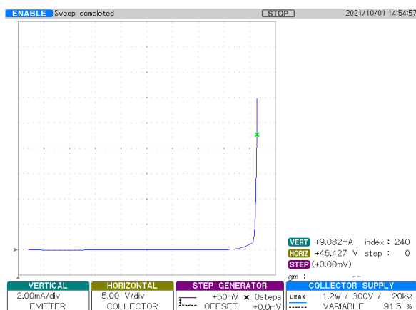
Figure 11. Typical V_S - V_{IS} Clamp Characteristic
