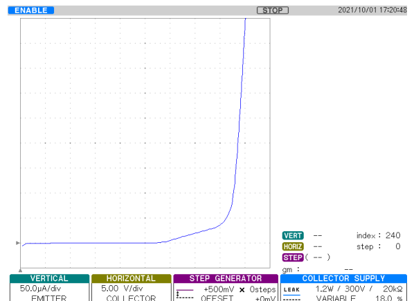
Figure 11. Typical V_S - V_{IS} Clamp Characteristic
