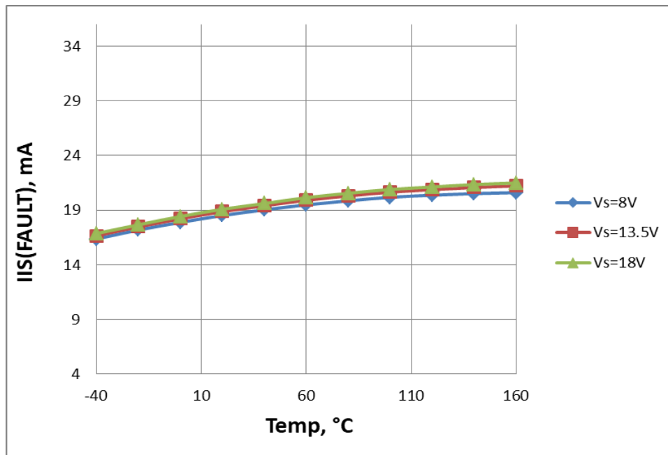
Figure 33. Sense Signal Maximum Current in Fault Condition I_{IS(FAULT)} = f(T_J; V_S)
