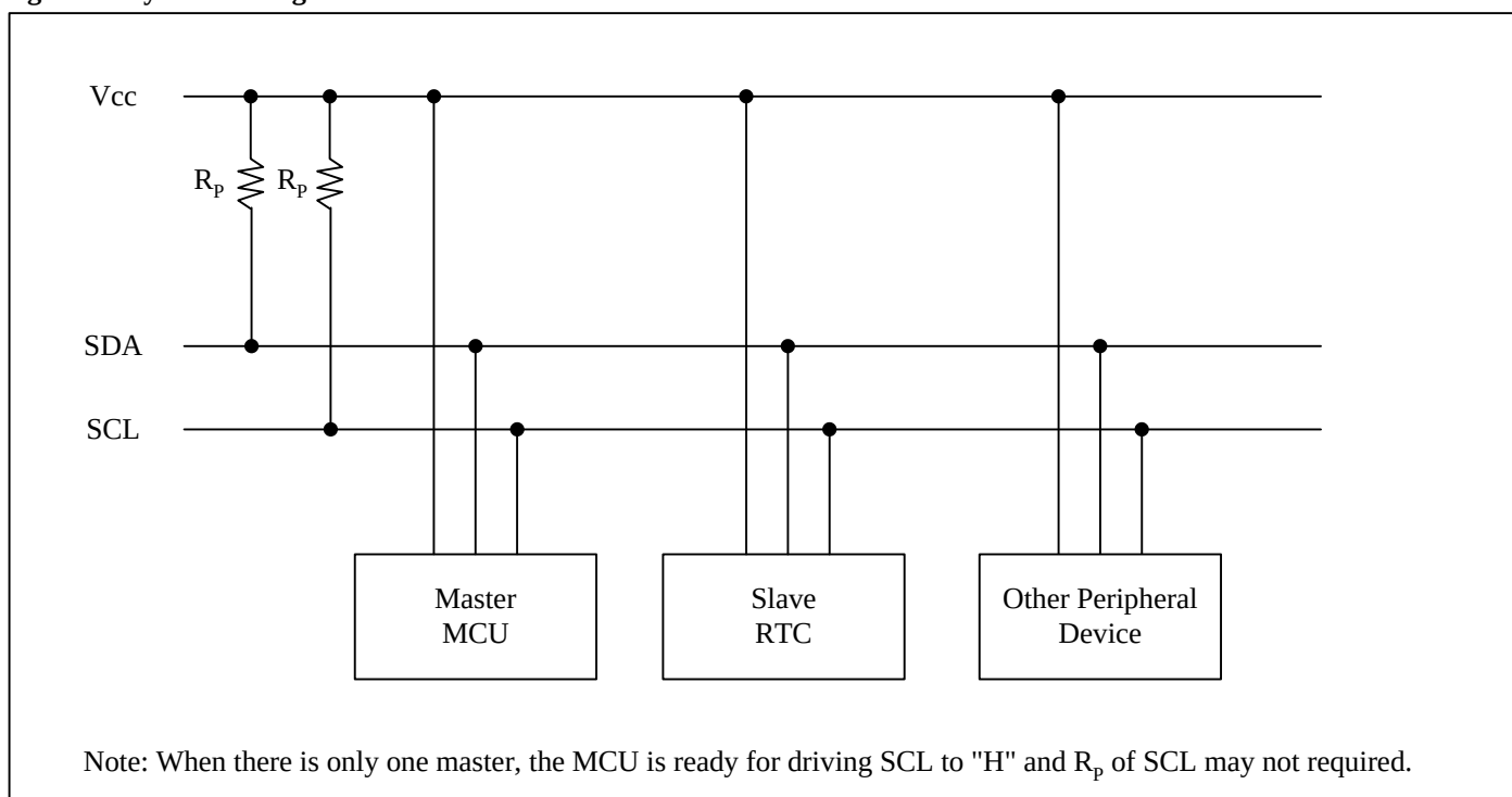
Figure 1. System Configuration
