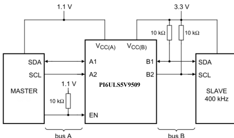
Figure 5. Typical Application
