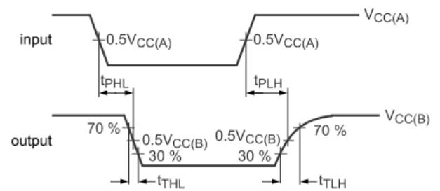
Figure 2. Propagation Delay and Transition Times A→B
