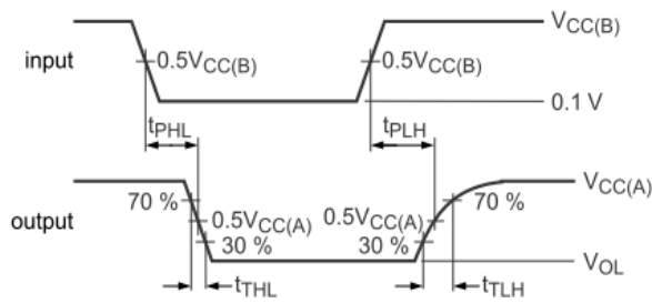
Figure 1. Propagation Delay and Transition Times B→A
