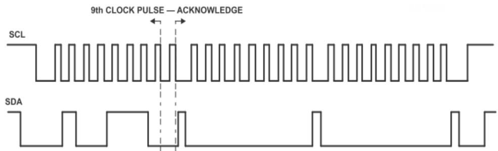
Figure 6. Bus B I²C/SMBus Waveform
