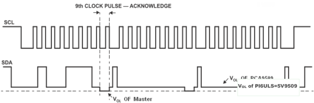
Figure 7. Bus A Lower Voltage Waveform
