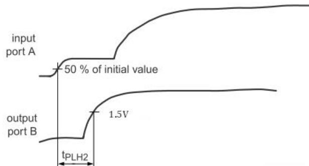
Figure 3. Propagation delay from the port A's external driver switching off to port B LOW-to-HIGH transition; (A→B)
