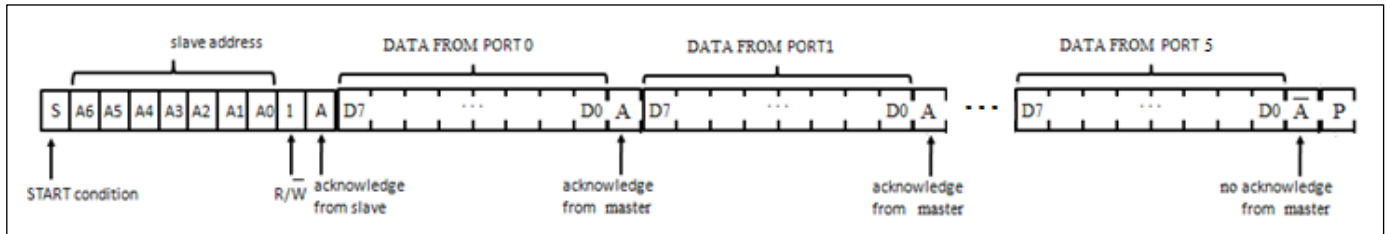
Figure 4. Read Input Port Register
