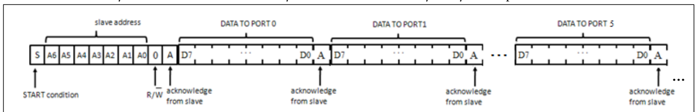
Figure 3. Write Mode
