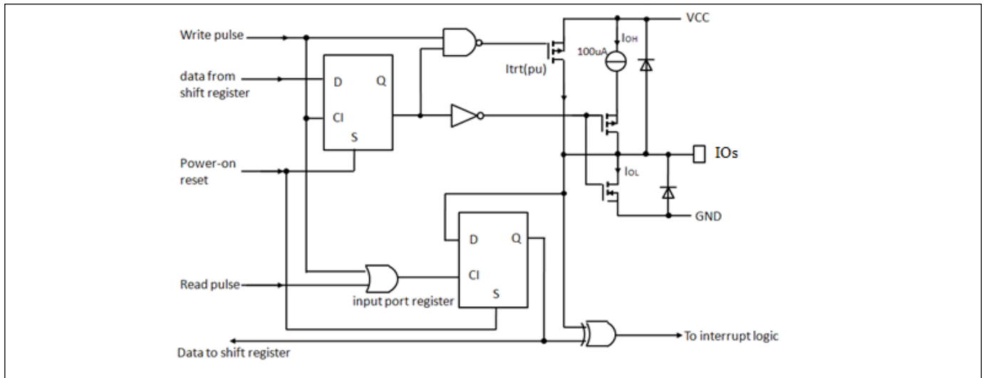
Figure 2. Simplified schematic diagram of IOX_0 to IOX_7
