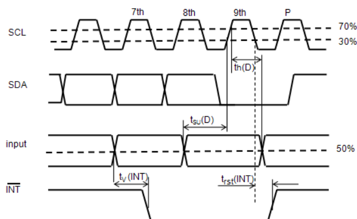
Figure 1. Timing Parameters for INT Signal
