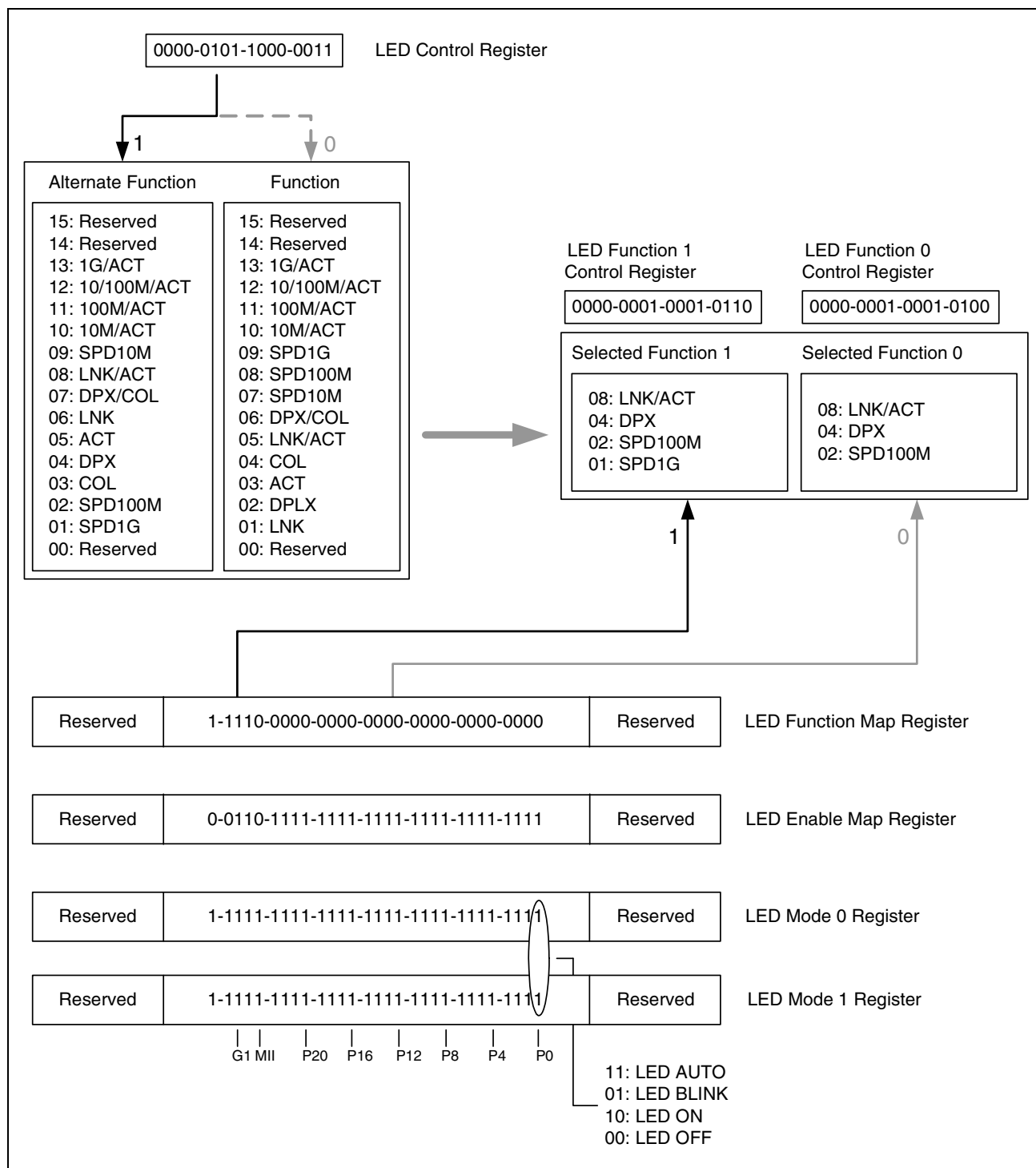
Figure 37: BCM53242 LED Register Structure Diagram
