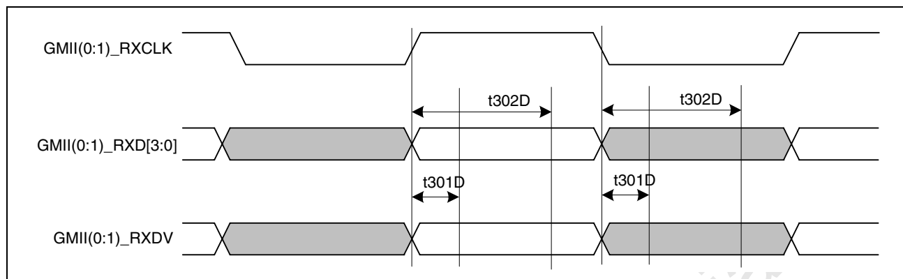
Figure 51: RGMII Input Timing (Delayed Mode Clock)
