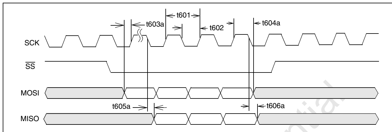
Figure 56: SPI Timing, \overline{SS} Asserted During SCK High
