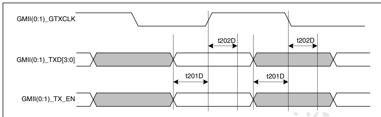
Figure 49: RGMI Output Timing (Delayed Mode Clock)
