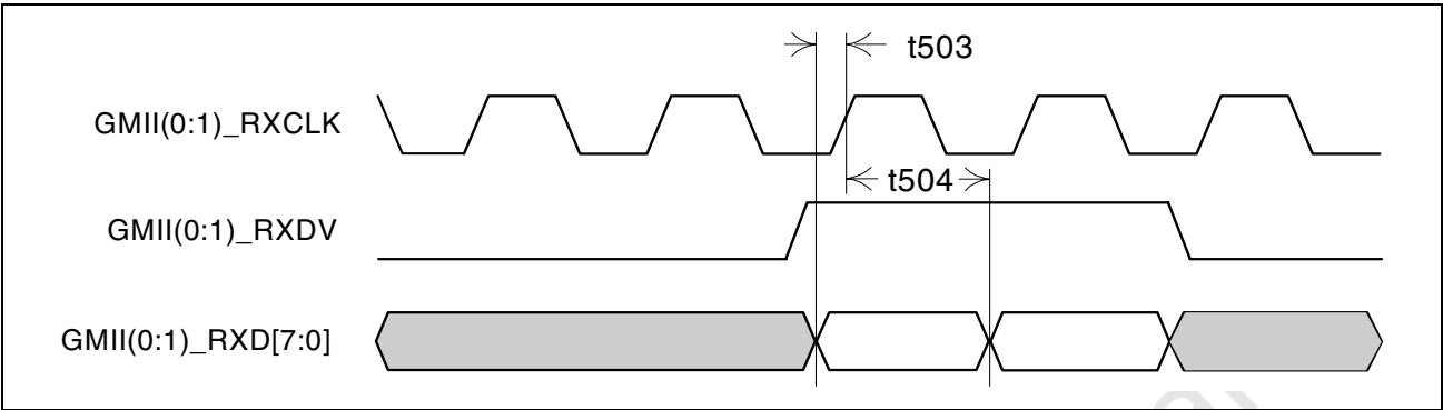
Figure 53: GMII Input Timing
