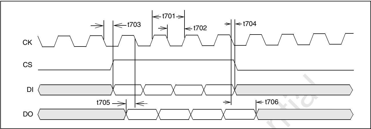
Figure 58: EEPROM Timing
