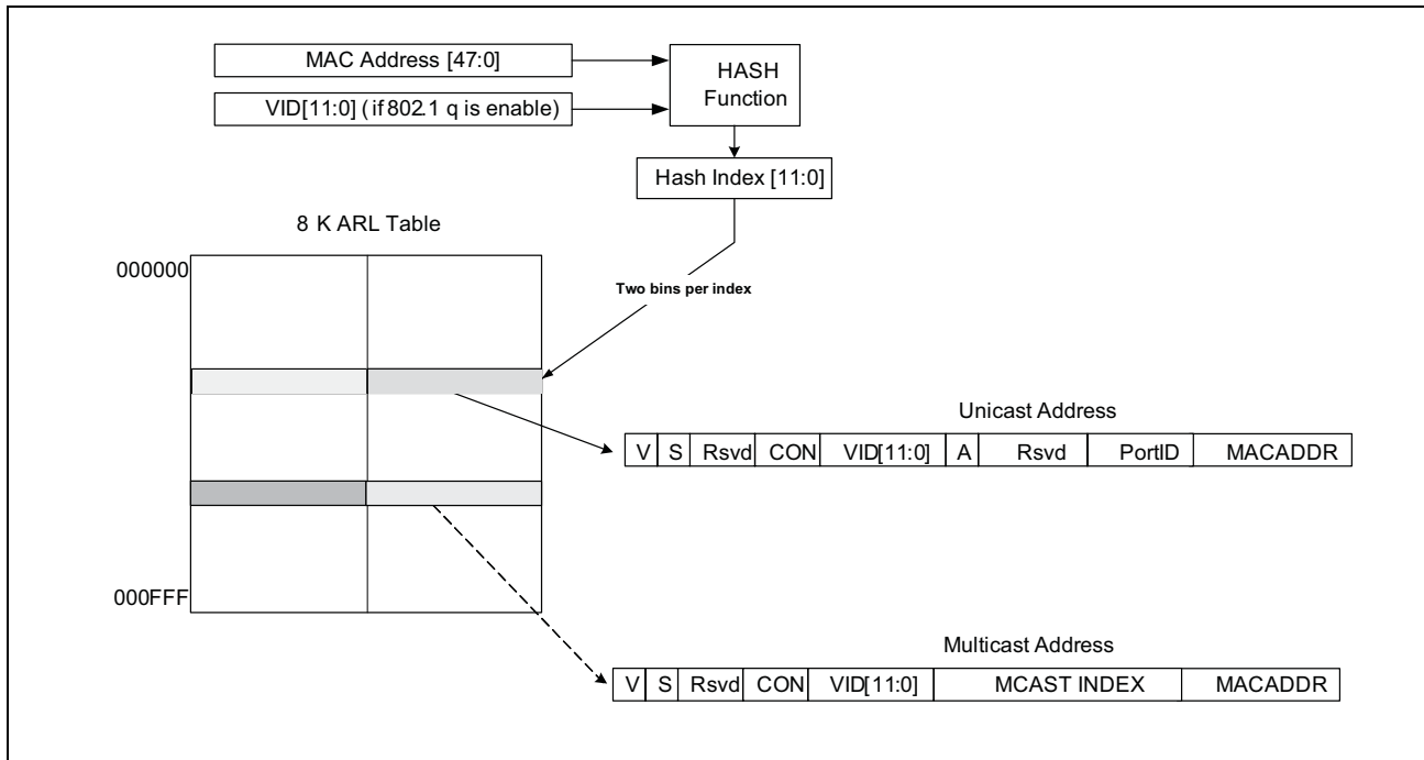
Figure 14: BCM53242M Address Table Organization
