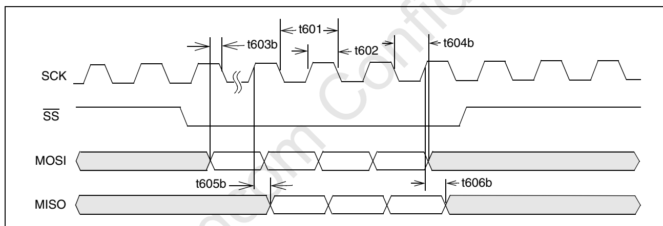
Figure 57: SPI Timing, \overline{SS} Asserted During SCK Low
