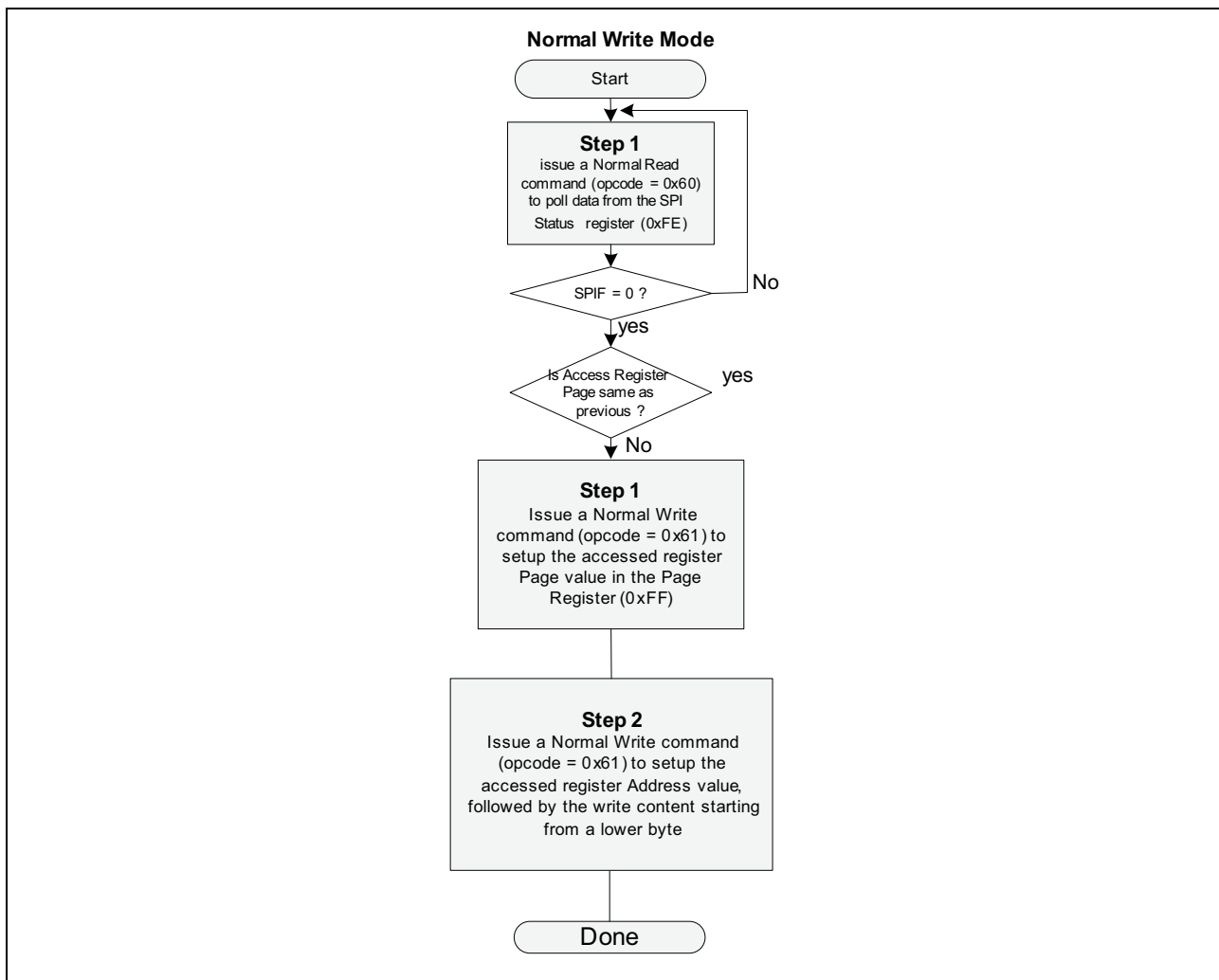
Figure 23: Normal SPI Mode Write Flow Chart
