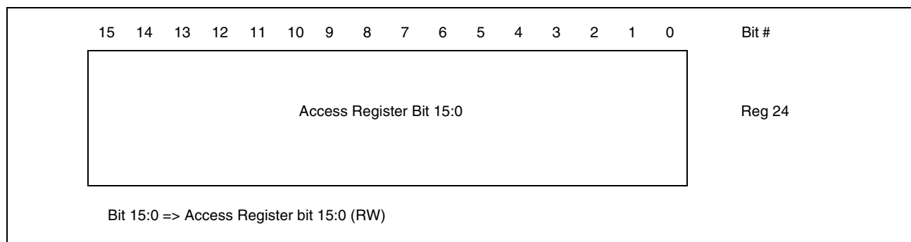
Figure 29: Pseudo PHY MII Register 24: Access Register Bit Definition
