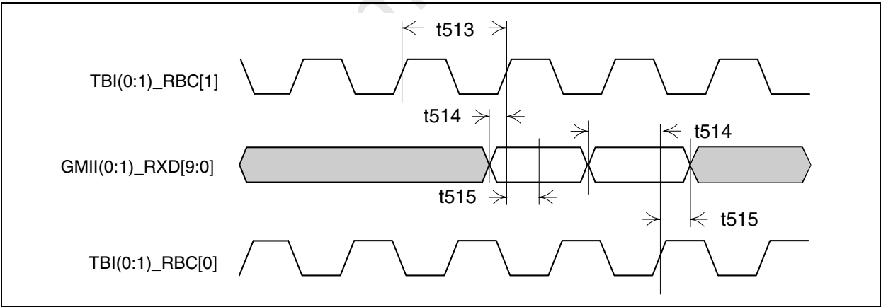
Figure 55: TBI Input Timing
